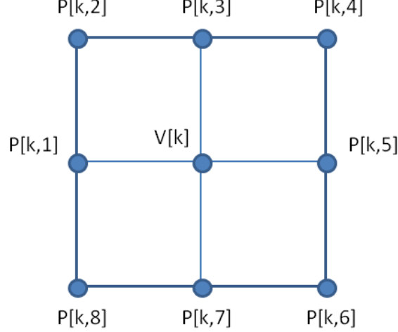
Figure 7: This figure illustrates how the neighboring vertices (forms set \mathbf{P}_k ) of a given vertex V[k] \in \mathbf{V} in a quad surface are ordered.
