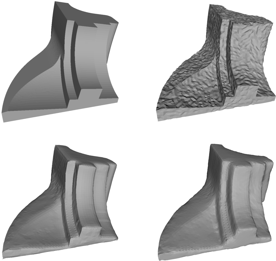
Figure 5: The fan disk model (top-left) is artificially corrupted by Gaussian noise ( \sigma = 1/5 of the mean edge length) (top-right), then smoothed by bilateral filtering (bottom-left) and Algorithm-Tri-1 (bottom-right).
