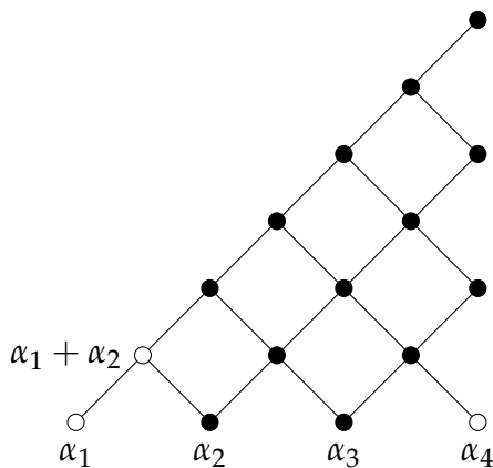
Figure 1: The root poset for type B_4 is shown, with the filled nodes indicating the positive roots in the inversion set of the element w from Example 1.
